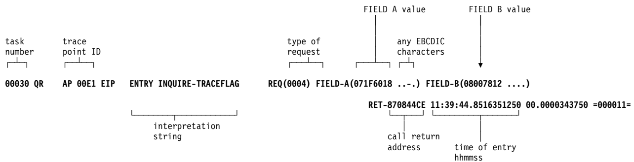
Figure 51. Example of the short-format for an old-style trace entry
