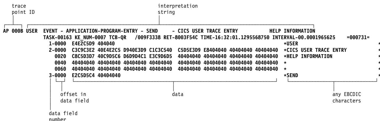
Figure 53. Example of the extended format for a user trace entry
