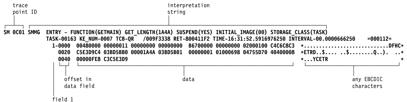
Figure 47. Example of the extended format for a new-style trace entry
