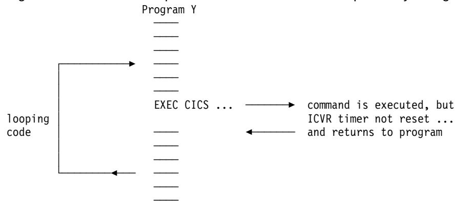
Figure 27. A non-yielding loop
