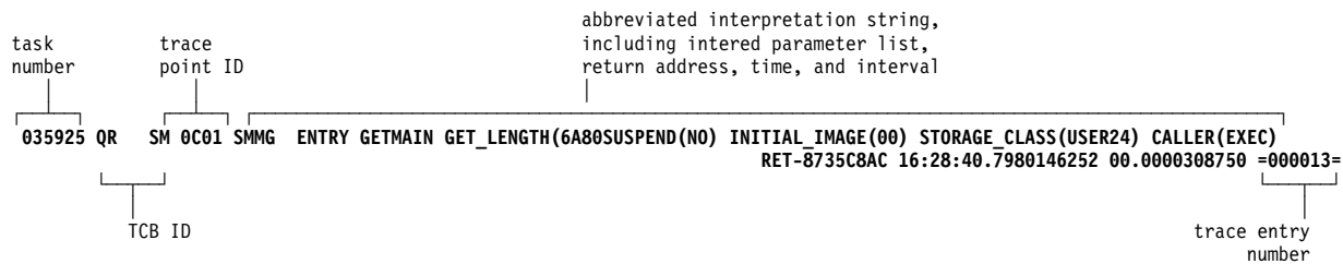
Figure 52. Example of the short-format for a new-style trace entry
