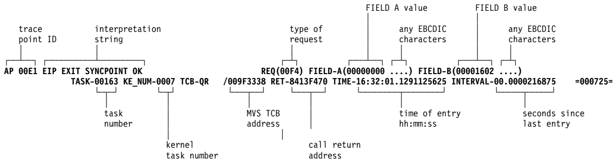
Figure 46. Example of the extended format for an old-style trace entry
