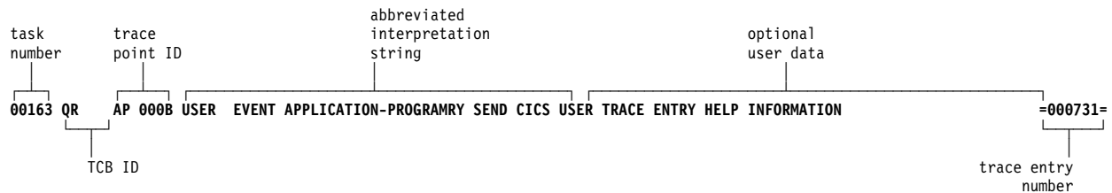
Figure 54. Example of the abbreviated format for a user trace entry
