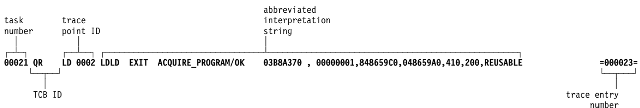
Figure 49. Example of the abbreviated format for a new-style trace entry
