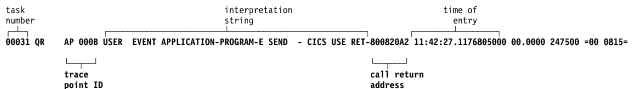
Figure 55. Example of the short format for a user trace entry
