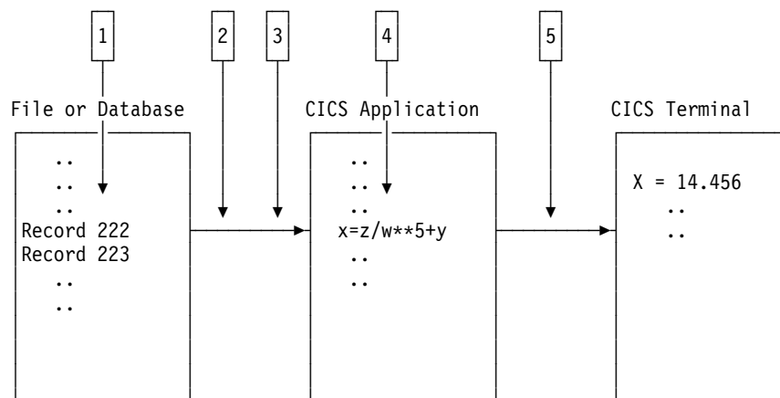
Figure 35. Where data might be corrupted in a transaction
